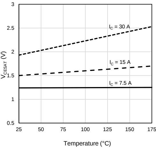
Figure 7: Collect-emitter saturation voltage vs. Junction Temperature
