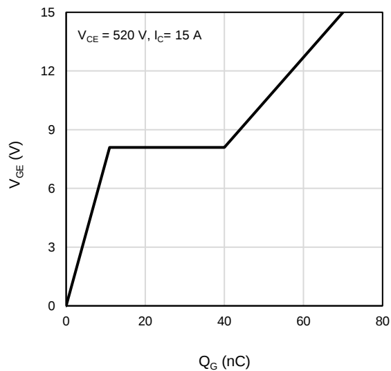
Figure 16: Gate-Charge Characteristics
