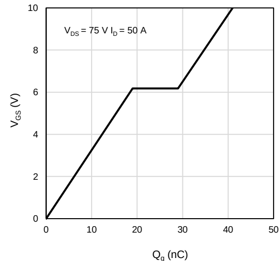
Figure 10: Gate-Charge Characteristics
