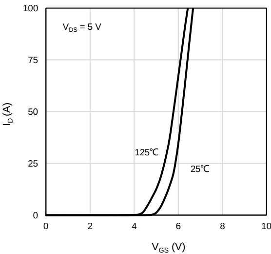
Figure 2: Transfer Characteristics
