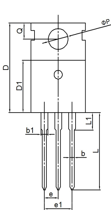
Top View
