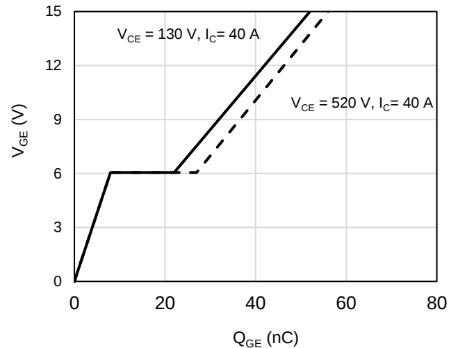
Figure 16: Gate-Charge Characteristics
