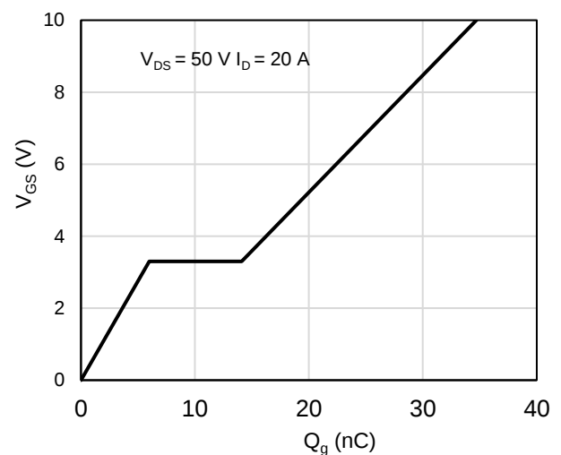
Figure 10: Gate-Charge Characteristics
