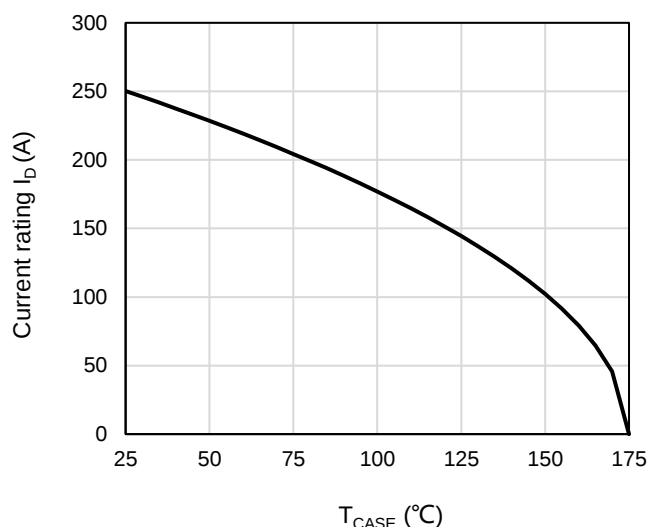
Figure 12: Current De-rating
