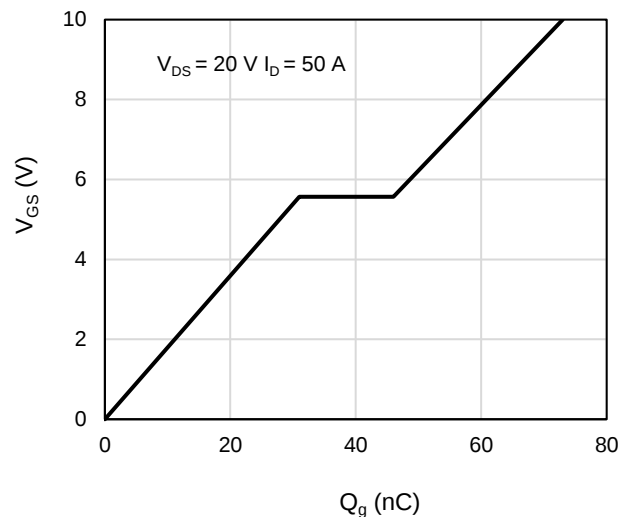
Figure 10: Gate-Charge Characteristics
