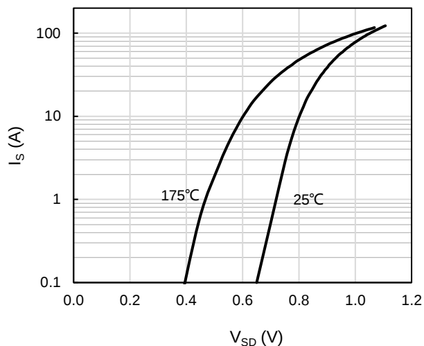
Figure 7: Body-Diode Characteristics
