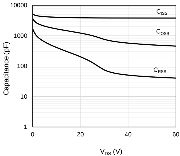
Figure 9: Capacitance Characteristics
