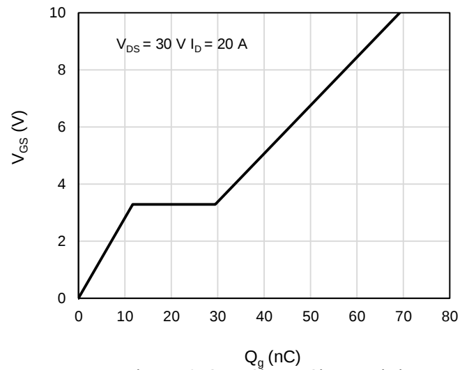
Figure 10: Gate-Charge Characteristics
