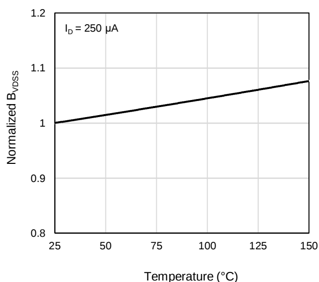
Figure 5: Breakdown Voltage vs. Junction Temperature
