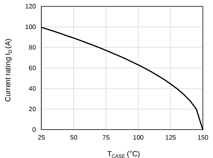
Figure 12: Current De-rating
