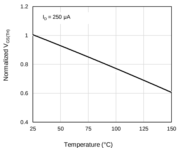
Figure 6: Threshold Voltage vs. Junction Temperature
